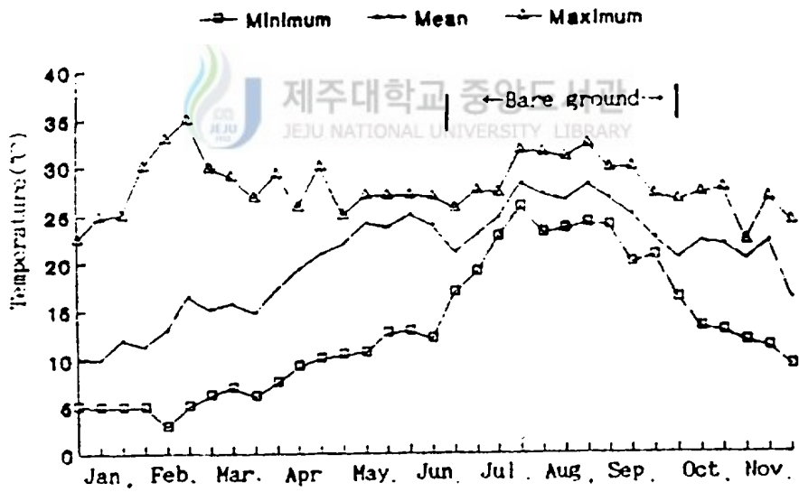
Fig. 2. Plastic film green house temperature
