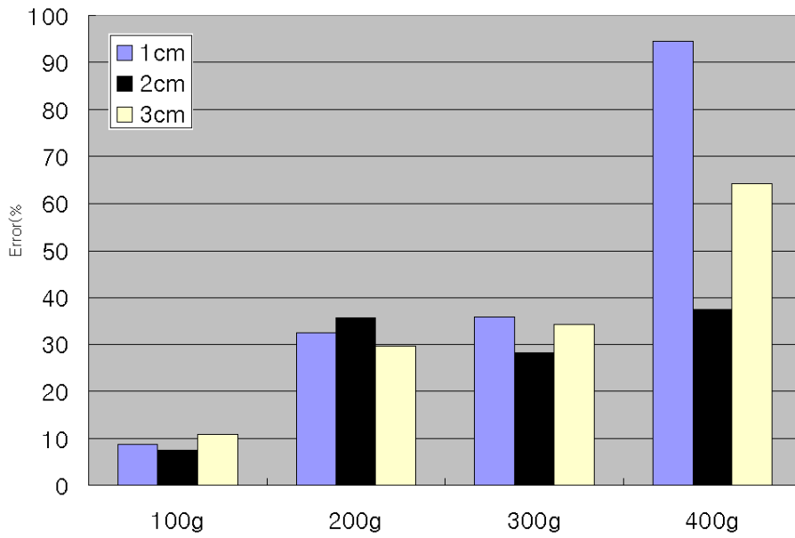
Fig. 2-14 Error characteristics according to buffer thickness ( Impact distance : 16cm, Belt speed : 1.5m/s )
