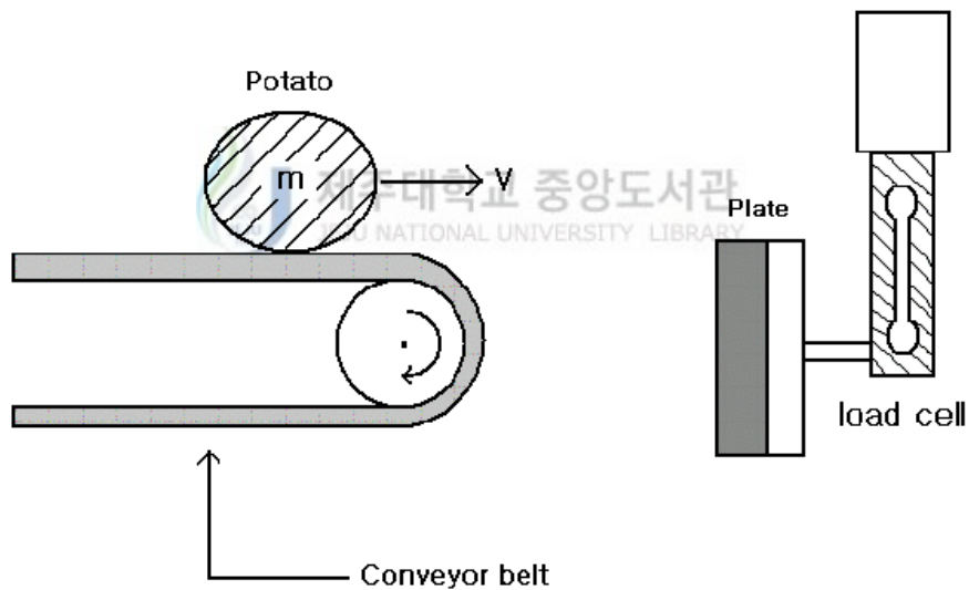
Fig. 2-7 Schematic diagram of the weighting system
