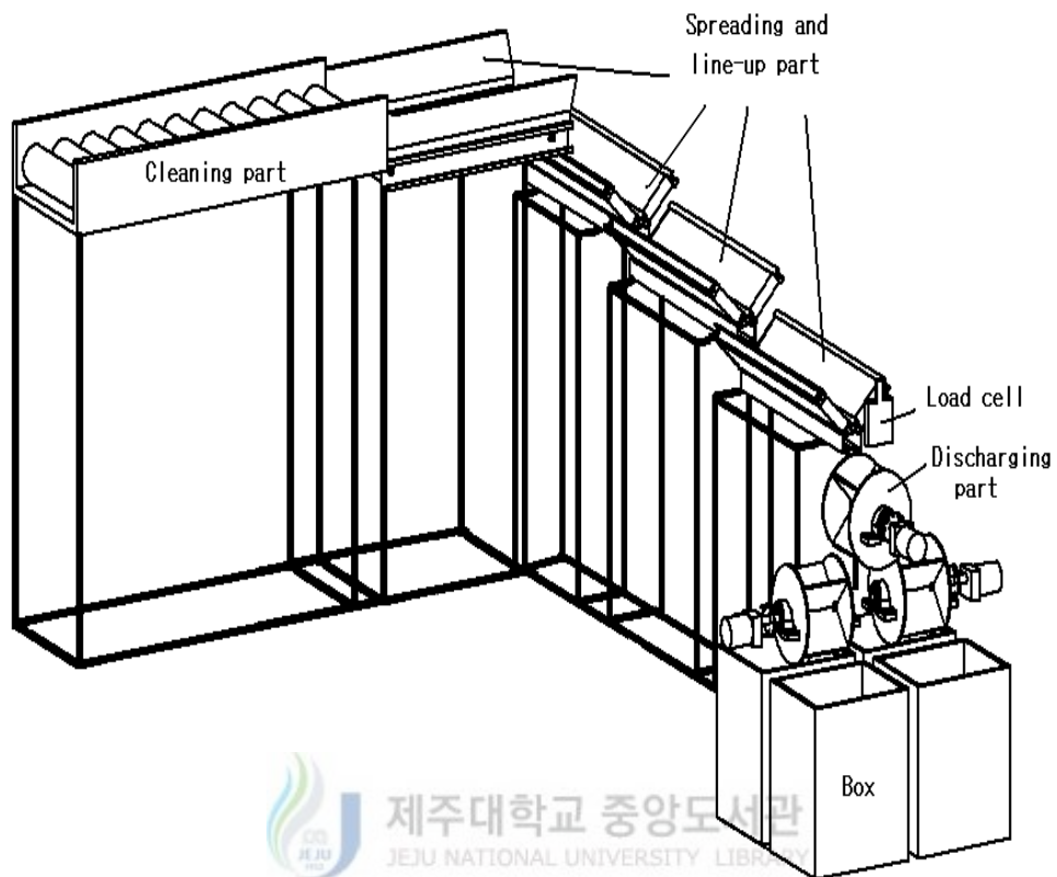
Fig. 3-1 Schematic diagram of the sorting system
