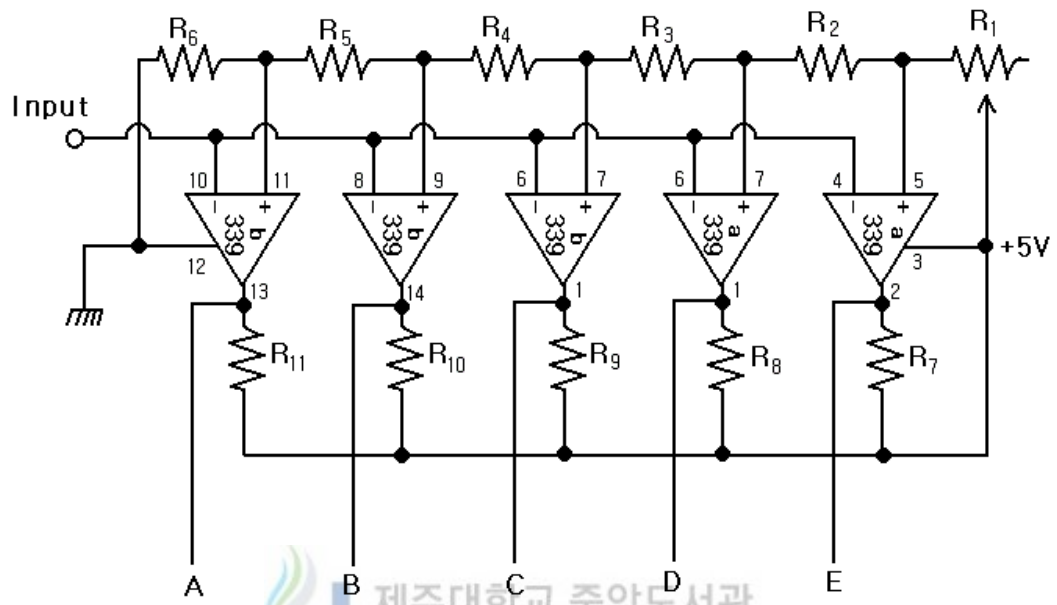
Fig. 2-10 Level detector circuit
