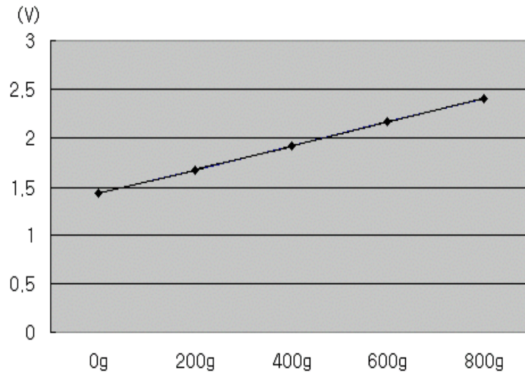
Fig. 2-6 Linear pattern of the load cell output
