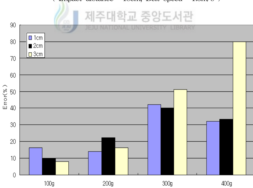
Fig. 2-13 Error characteristics according to buffer thickness ( Impact distance : 18cm, Belt speed : 1.5m/s )
