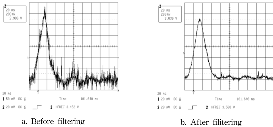
Fig. 2-5 Effect of the filter
