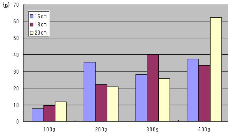
Fig. 2-16 Error characteristics according to impact distance ( Belt speed : 1.5m/s, Buffer thickness : 2cm )
