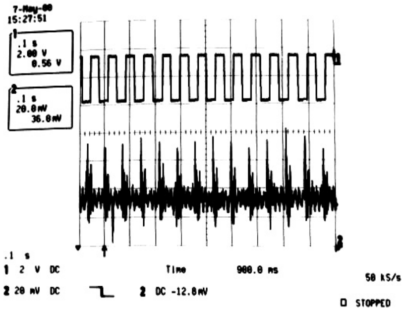
Fig. 2-3 Response characteristics of the load cell
