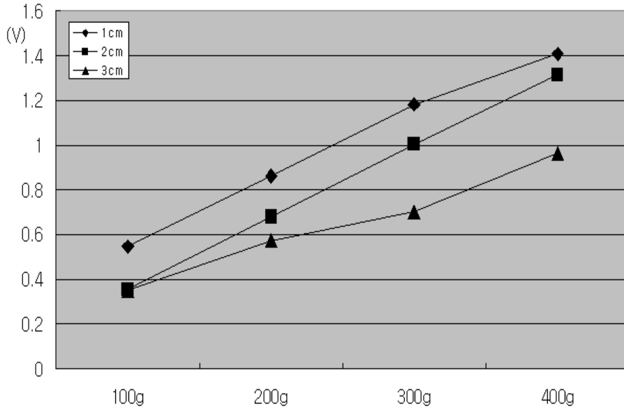
Fig. 2-12 Output characteristics according to buffer thickness ( Impact distance : 18cm, Belt speed : 1.5m/s )
