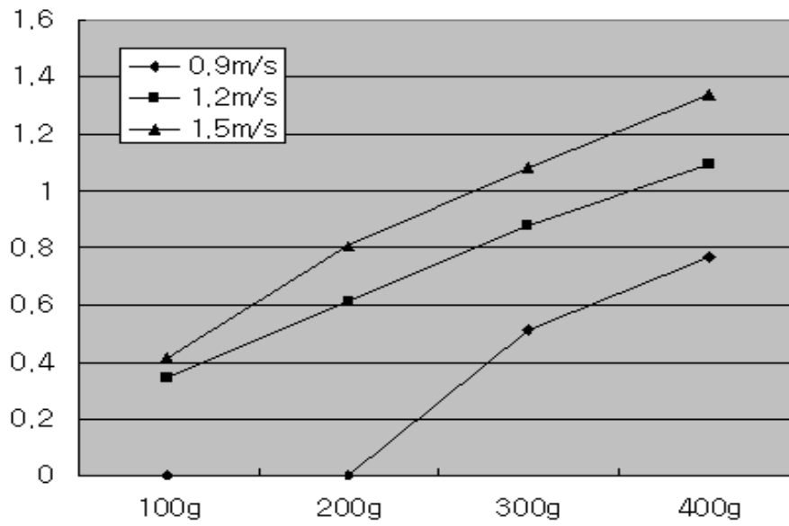
Fig. 2-11 Output characteristics according to belt speed ( Buffer thickness : 2cm, Impact distance : 16cm )
