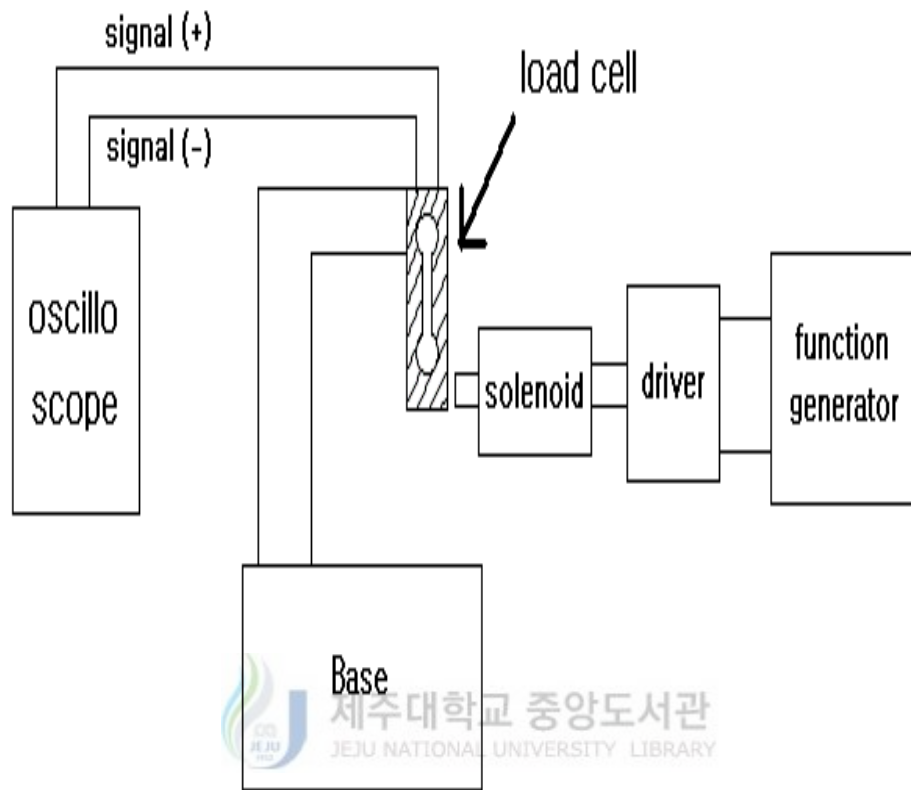
Fig. 2-2 Experimental set-up for testing the load cell
