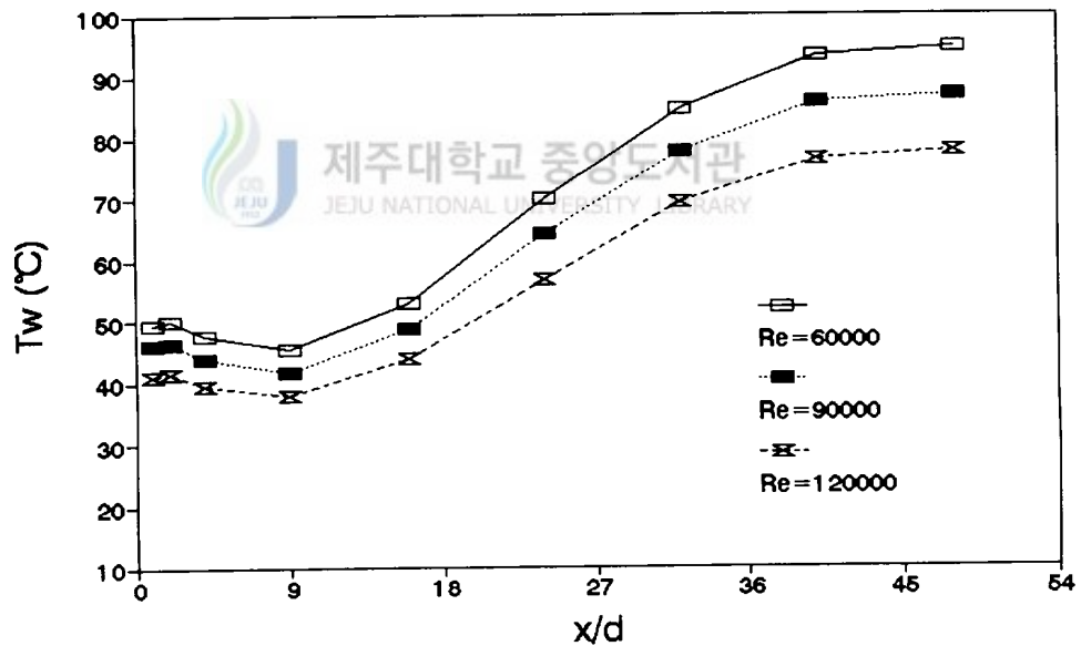
Fig.15 Distribution of wall temperature along the downstream for various Reynolds numbers
