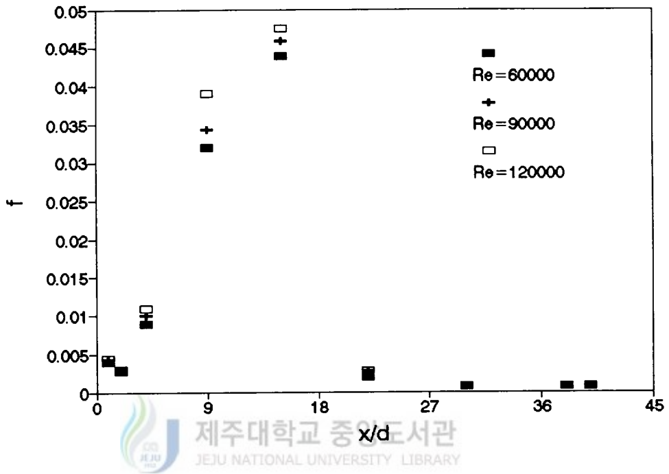
Fig.13 Friction factors distribution for various Reynolds numbers with an 10°-inclined concentric expansion
