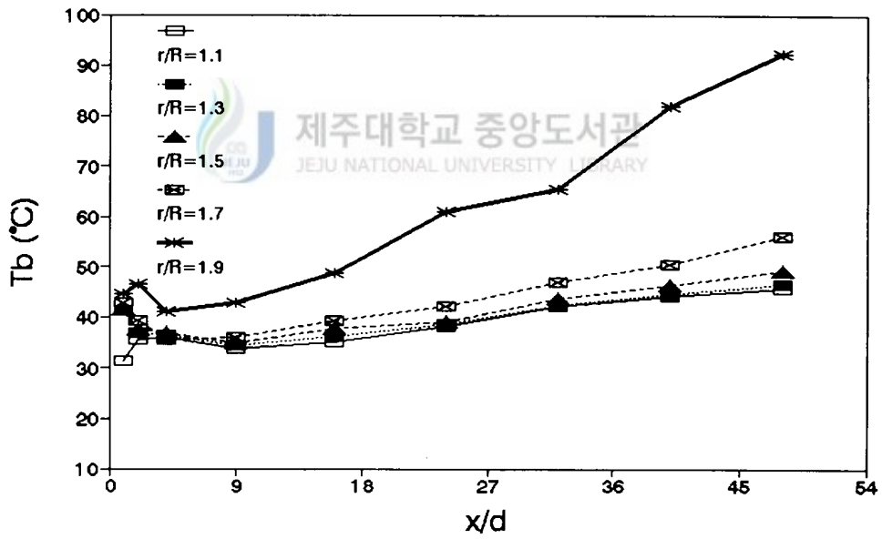
Fig.19 Distribution of bulk temperature along the downstream for Re=60,000
