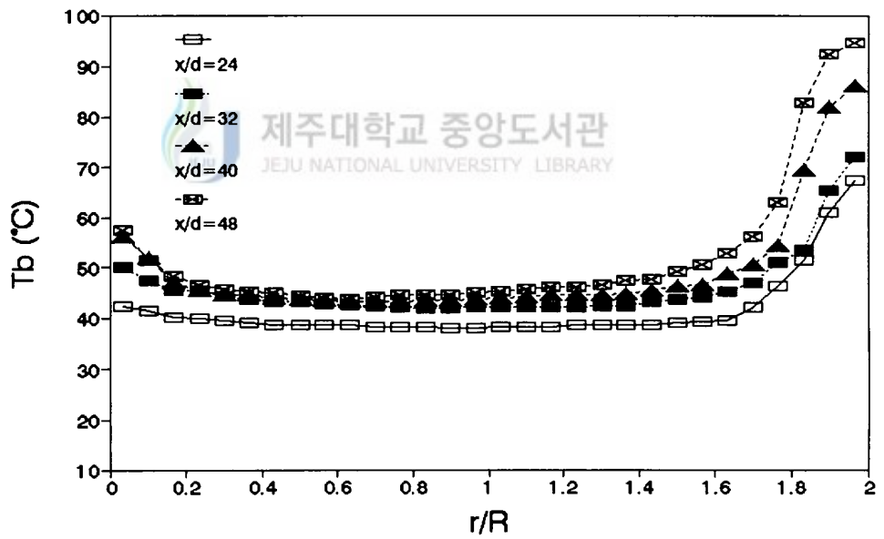
Fig.16 Distribution of bulk temperature along the downstream for Re=60,000
