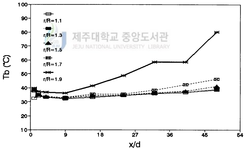
Fig. 20 Distribution of bulk temperature along the downstream for Re=90,000
