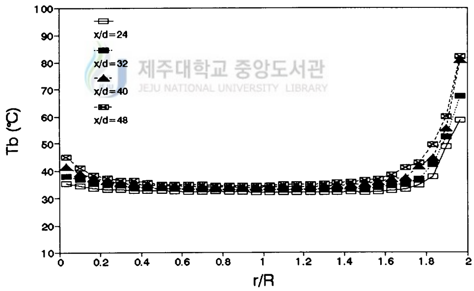
Fig.18 Distribution of bulk temperature along the downstream for Re=120,000
