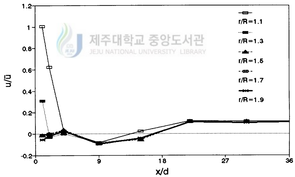
Fig.10 Streamlines and steady flow from r/R=0.1 to 1.9 for Re=90,000 with an inclined concentric expansion
