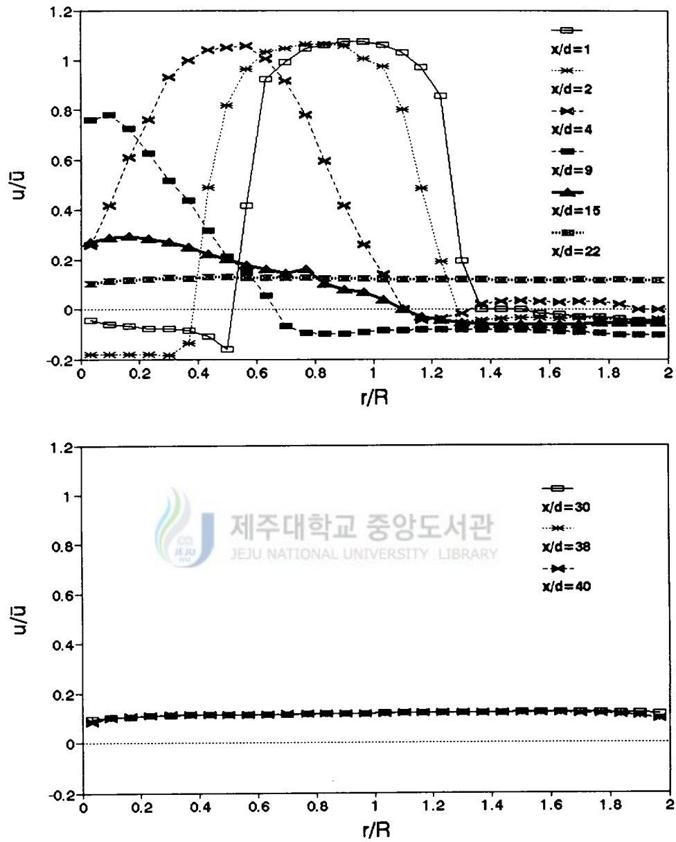
Fig.8 Axial velocity profiles for Re=120,000 with an inclined concentric expansion
