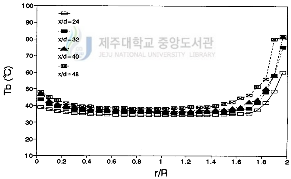
Fig. 17 Distribution of bulk temperature along the downstream for Re=90,000
