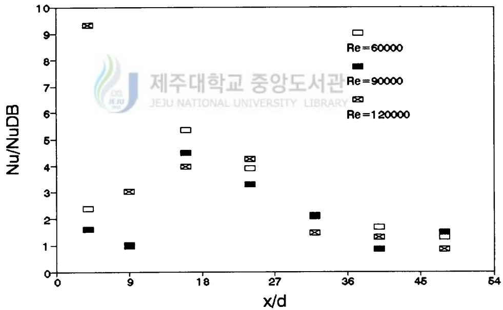
Fig. 22 Distribution of Nu/Nu_{DB} along the downstream for various Reynolds numbers with an 10^\circ -inclined concentric expansion
