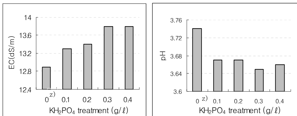
Fig 9. Effects of \text{KH}_2\text{PO}_4 treatment on pH and EC in the closed ebb and flow system.
