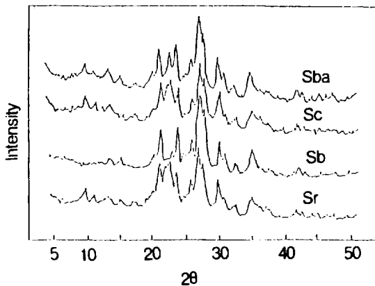
Fig. 3. The X-ray diffraction patterns of variously chemically treated natural zeolite S.
