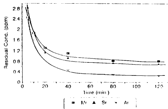
Fig. 5. Removal isotherm of Sr(II) ion using the untreated natural zeolite Mr, Sr, and Ar.
