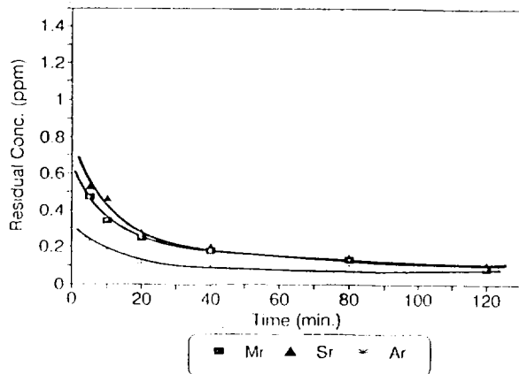
Fig. 4. Removal isotherm of Cs(I) ion using the untreated natural zeolites Mr, Sr, and Ar.
