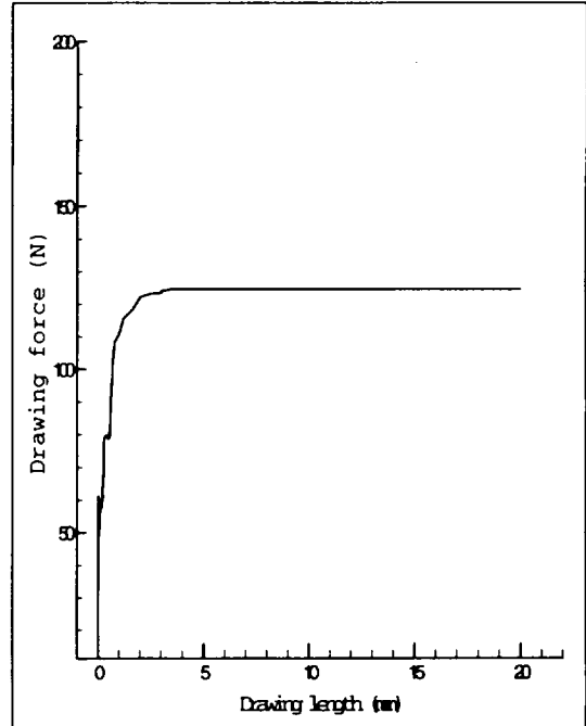
Fig. 7. Variation of drawing force according to the drawing displacement.
