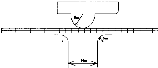
Fig. 2. Shape of the die and the circular bead punch.
