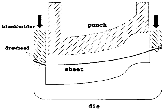
Fig. 1. Schematic diagram of a general blank forming process.
