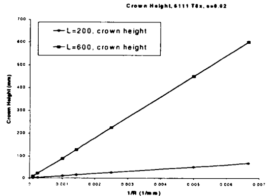
Fig. 3. Crown height as a function of curvature.
