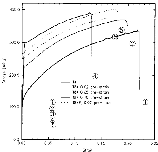
Fig. 2. Stress-strain curves adopted for the sheet materials.
