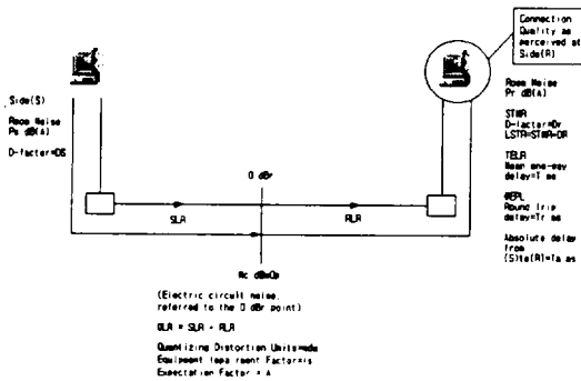
Fig. 4. E-Model Reference Diagram.
